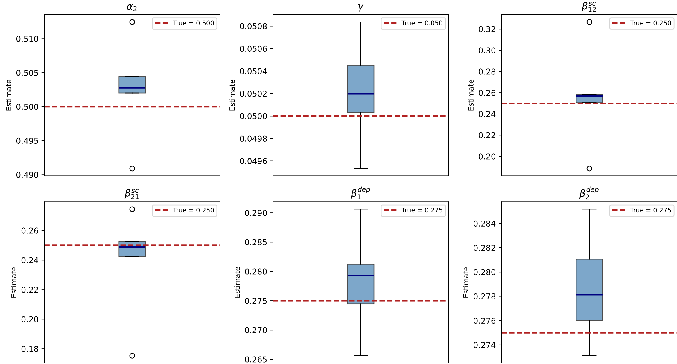
NFXP Monte Carlo: original model ( \beta^{dep} brand-specific) (reps=5, N=2000, T=52)
